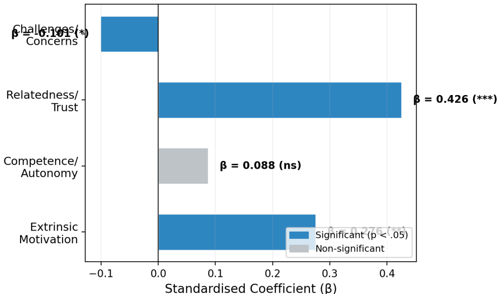
MLR: Predictors of ChatGPT Utilisation ( R^2 = 0.563 , N = 202)
