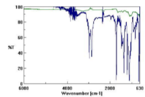
Fig.5 Cladophora and retinol Spectre IR
