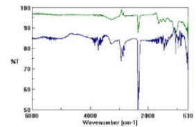
Fig.3 Cladophora and calciferol Spectre IR
