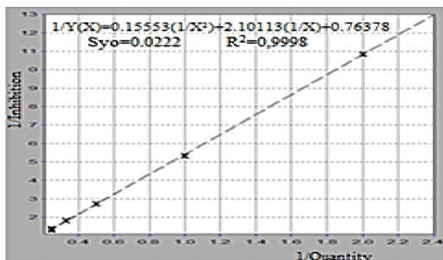
Figura 13. Calibration curve for standard Trolox (ACL method, Analytik Jena, Germany)
