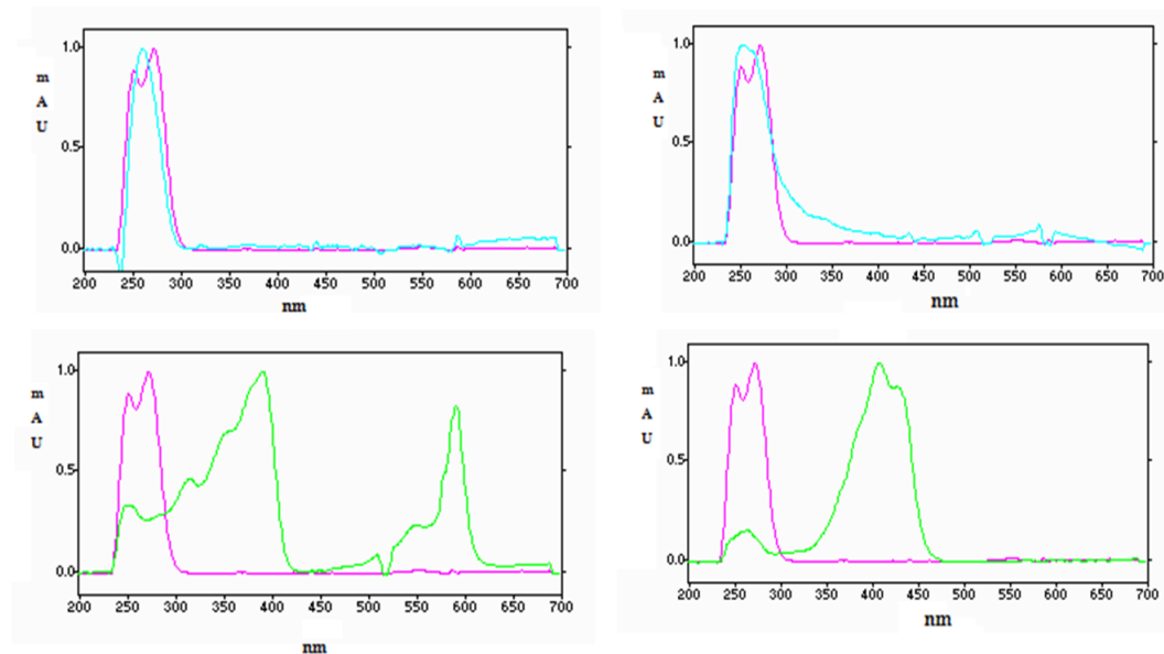
Figure 4. The chromatogram for Ceramium rubrum 0,5 mg/mL
