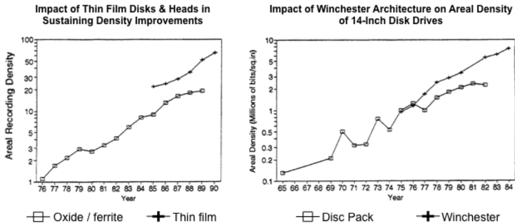
Figure 5: Example of sustaining technological change in componentry (left) and product architecture (right)
