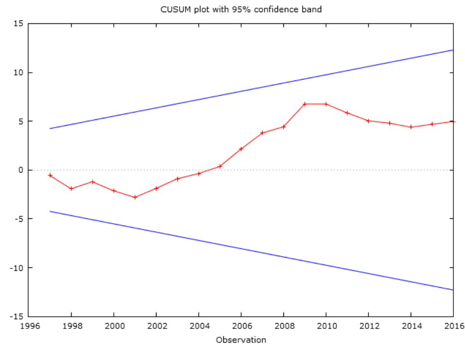
Graph 1. CUSUM test results.
