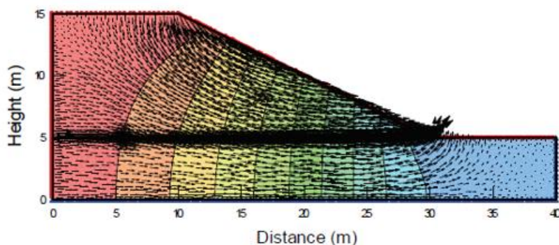
Fig.3.4 Flow field and equipotential lines from SEEP/W
